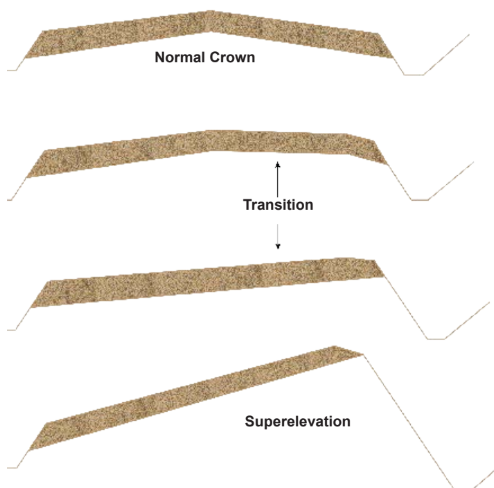
FIGURE 10: Crown to superelevation transition.
